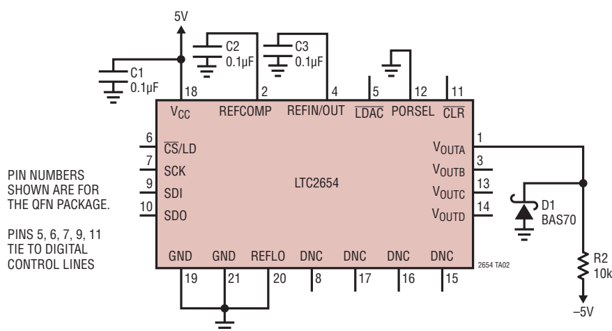
True Rail-to-Rail Output DAC
